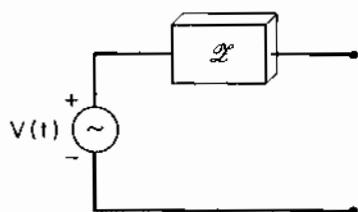
Figure 10.3 Thevenin Equivalent Circuit for Which the Spectral Density S_V(f) of the Voltage V Is Specified by (10.97)
