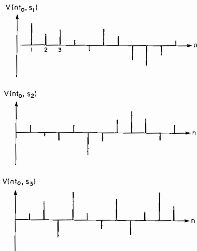
Figure 3.4 Statistical Samples of a Discrete-Time Random Process
