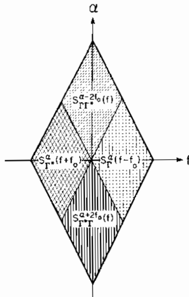
Figure 12.14 Support Regions for the Spectral Correlation Functions Associated with the Complex Envelope of a Bandlimited Signal (Exercise 8).
