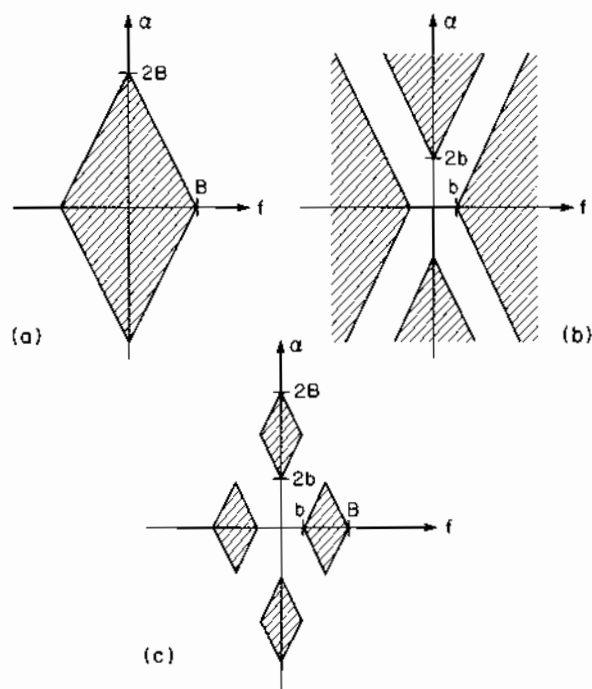
Figure 12.1 Support for Cyclic Spectra of Mean-Square Bandlimited Processes; (a) Low-pass, (b) High-pass, (c) Bandpass
