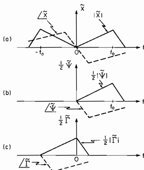
Figure 11.3 Equivalent Signal Representations in the Frequency Domain
