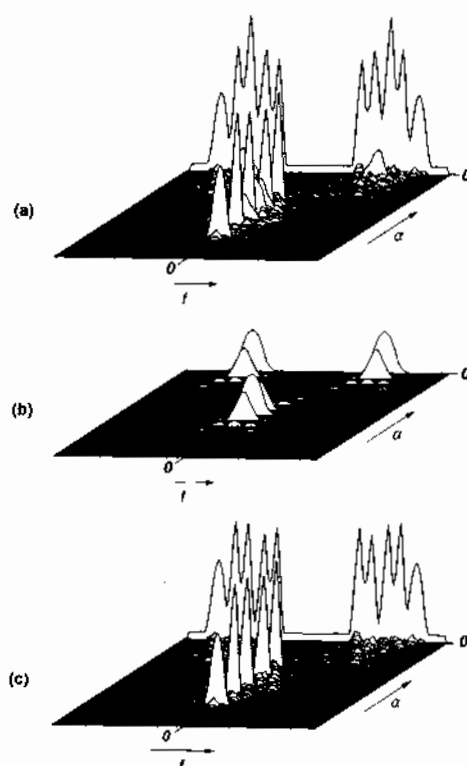
Figure 12.8 (a) Magnitude of Spectral Correlation Surface Computed from a Simulated BPSK Signal with Multiple AM Interference and Noise. (b) Same as (a) Except Signal Only. (c) Same as (a) Except Interference and Noise Only.
