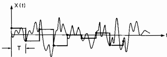
Figure 4.3 Statistical Sample of the Sampled-and-Held Noise Process
