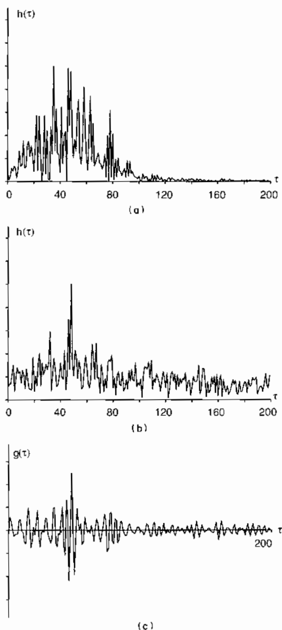
Figure 12.10 (a) Graph of the Conventional Generalized Cross-Correlation Function for a Segment of Length 2048T_c of the Corrupted Signal with the Spectrum and Cyclic Spectrum Shown in Figure 12.8a. (b) Graph of the Generalized Cross-Correlation Function from the SPECCORR Method for the Same Corrupted Signal Segment as in Part (a). (c) Graph of the Function (12.229) From the SPECCORP Method for the Same Corrupted Signal Segment as in Part (a).
