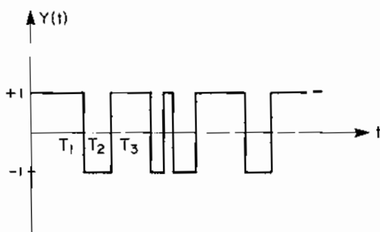
Figure 6.7 Statistical Sample of the Asynchronous Telegraph Signal
