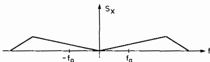
Figure 11.11 Spectral Density of X(t) for Exercise 6(c)
