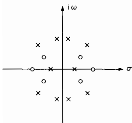
Figure 13.5 Typical Pole-Zero Diagram for Bilateral Laplace Transform \bar{S}_Y(s) of an Autocorrelation Function, Illustrating Quadrantal Symmetry
