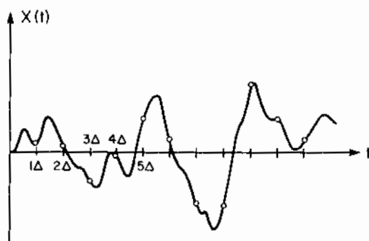
Figure 8.1 Equally Spaced Time Samples of a WSS Process
