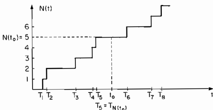
Figure 6.4 Statistical Sample of the Poisson Counting Process
