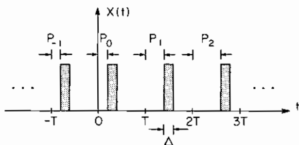
Figure 4.5 Statistical Sample of a Pulse-Position-Modulated Signal
