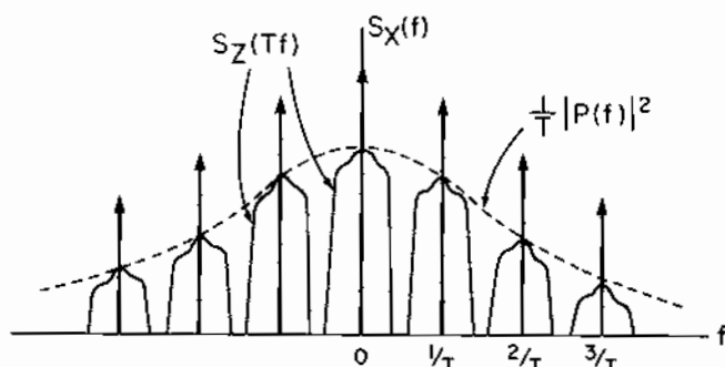
Figure 11.2 Power Spectral Density (11.8) for the Physical Manifestation of a Discrete-Time Process
