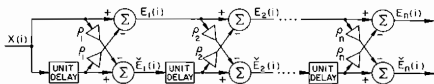
Figure 11.10 Lattice Implementation of Prediction Error Filter
