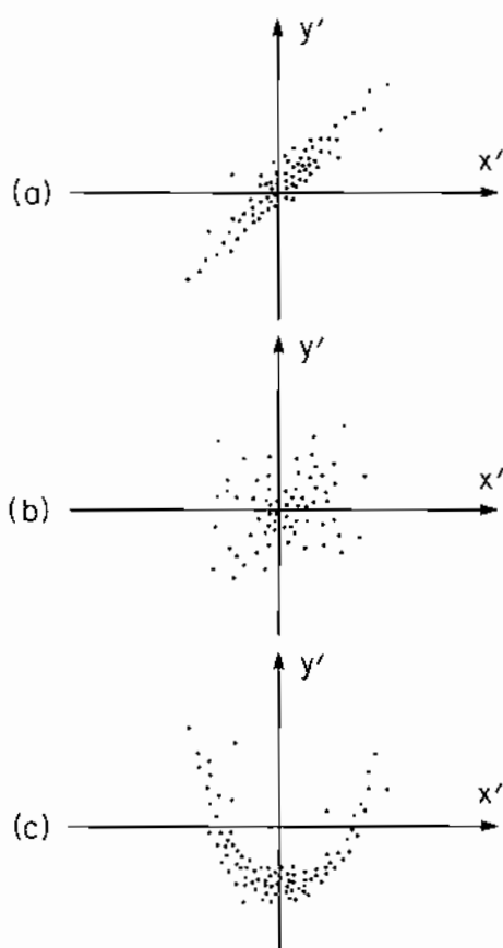
Figure 2.2 Examples of Scatterplots
