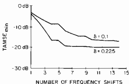
Figure 12.13 Theoretical MSE Performance of Optimum FRESH Filter Versus the Number of Frequency Shifts Used for Two Interfering AM Signals in Noise. The Parameter \delta is the Bandwidth-normalized Carrier Offset between the Two Signals.
