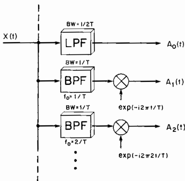
Figure 12.7 Decomposition of Cyclostationary Process into Stationary Components by Frequency-Division Demultiplexing Operation
