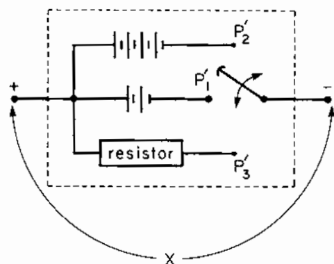
Figure 1.12 Example of a Mixed Random Variable
