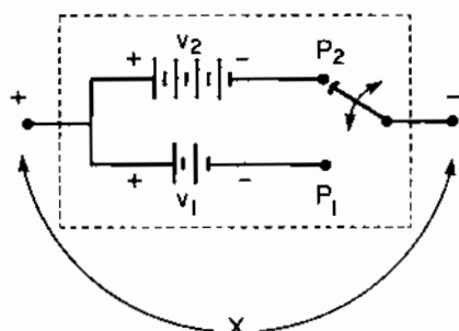
Figure 1.9 Randomly Selected Battery: An Example of a Discrete Random Variable
