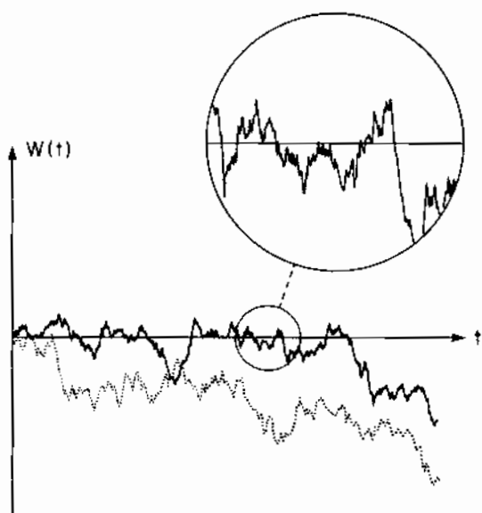
Figure 6.3 Two Statistical Samples of the Wiener Process
