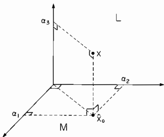
Figure 13.2 Graphical Illustration of Orthogonal Projection \hat{X}_0 of X \in L onto M
