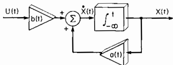
Figure 9.6 Block Diagram for Example 7
