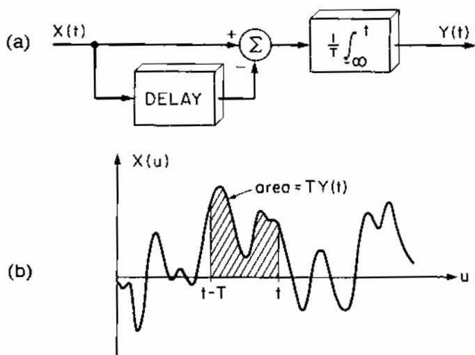
Figure 9.4 (a) Block Diagram of an Implementation of the Sliding-Window Smoother of Example 3; (b) Graphical Illustration of Sliding-Window Smoothing Operation
