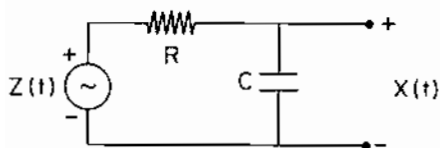
Figure 9.5 Circuit Diagram for Example 4
