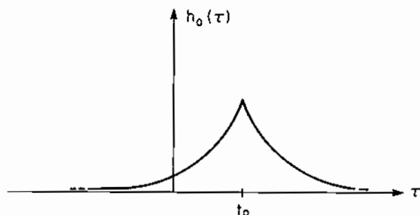
Figure 13.3 Optimum Impulse-Response Function for Example 2
