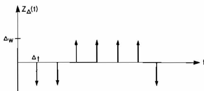
Figure 6.1 Statistical Sample of the Continuous-Time (Impulsive) \pm 1 Bernoulli Process
