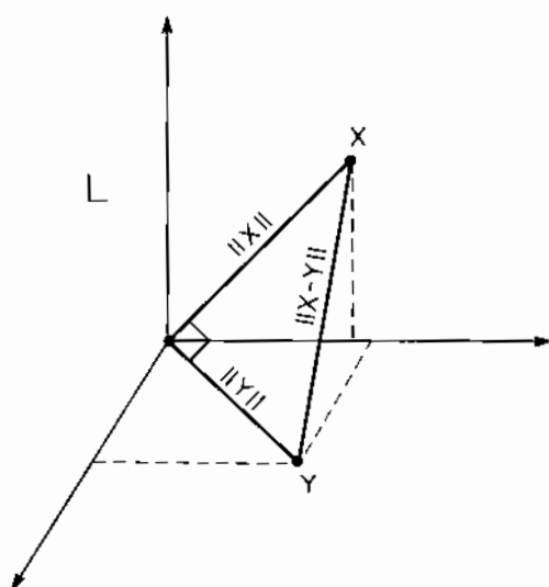
Figure 13.1 Graphical Illustration of Pythagorean Theorem for Vectors
