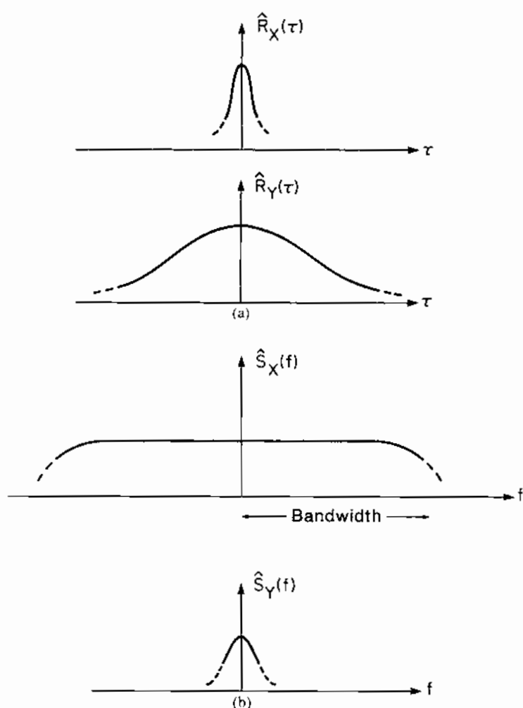
Figure 3.2 (a) Autocorrelation Functions; (b) Power Spectral Densities for Broadband and Narrowband Waveforms
