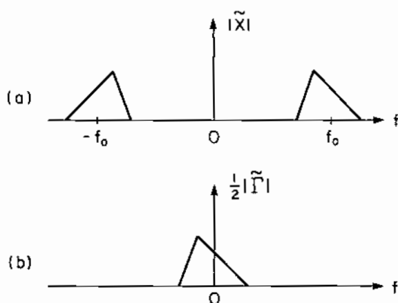
Figure 11.4 Low-Pass Representation of a Bandpass Signal
