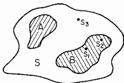
Figure 1.4 Pictorial Abstraction of Sample Space ( S ), Event Sets ( A, B ), and Sample Points ( s_1, s_2, s_3 )
