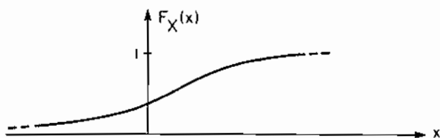
Figure 1.7 Example of a Probability Distribution Function
