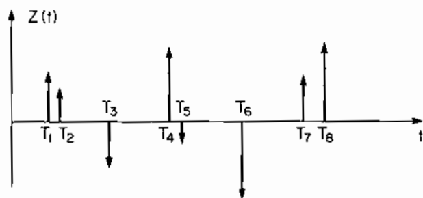
Figure 6.5 Statistical Sample of a Randomly Weighted Poisson Impulse Process
