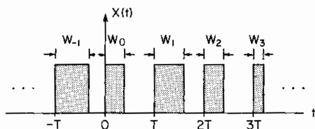
Figure 4.6 Statistical Sample of a Pulse-Width-Modulated Signal
