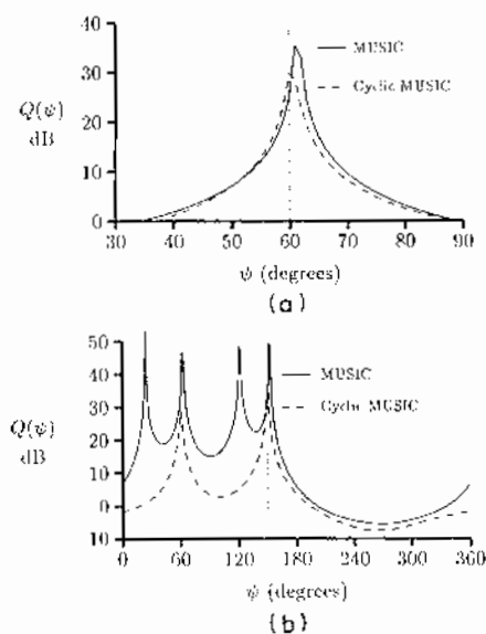
Figure 12.9 (a) Graphs of the DOA Estimation Function Q(\psi) in (12.213) for the MUSIC and Cyclic MUSIC Methods Applied to a Four-Element Circular Array with One Signal of Interest and One Interference. (b) Graphs of the DOA Estimation Function Q(\psi) in (12.213) for the MUSIC and Cyclic MUSIC Methods Applied to a Four-Element Circular Array with Two Signals of Interest and Three Interferences.
