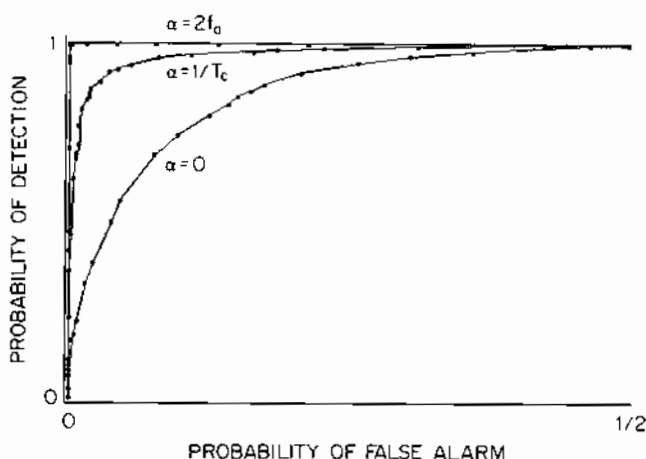
Figure 12.12 Graphs of Probability of Detection Versus Probability of False Alarm Computed From Simulations for Two Single-Cycle Detectors and the Radiometer. The Signal is BPSK and the Noise is White with Random Spectral Intensity Having Coefficient of Variation of 1/10 . The Average SNR is 0 dB and the Time-Bandwidth Product of the Signal is 256.
