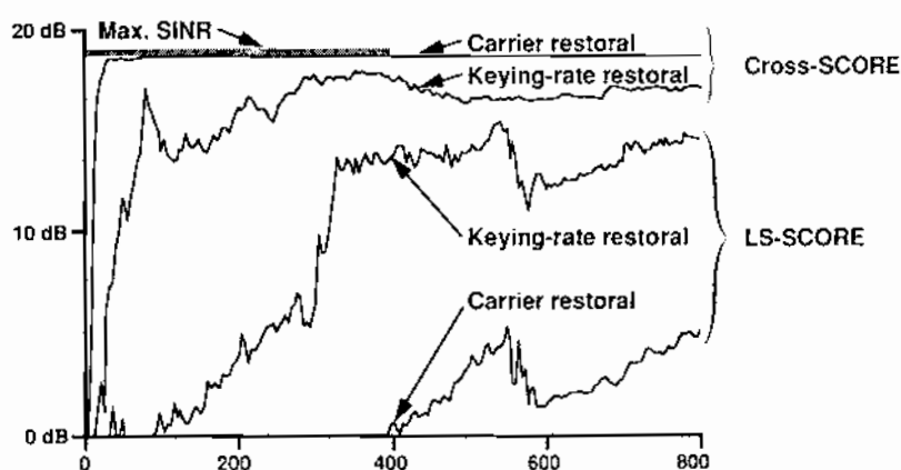
Figure 12.11 Graphs of the Output SINR Versus the Adaptation Time of the LS-SCORE and Cross-SCORE Algorithms.
