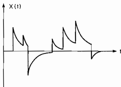
Figure 6.6 Statistical Sample of a Marked and Filtered Poisson Process with Causal Pulses
