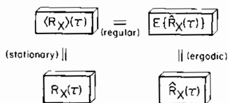
Figure 8.3 Relationships among Empirical and Probabilistic Autocorrelations
