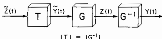
Figure 13.4 Relationship between a White Process \tilde{Z} and the Innovations Process Z
