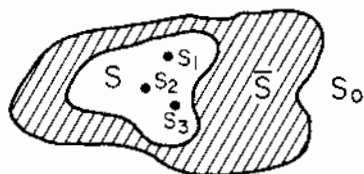
(a) Set containment and complement
