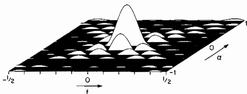
Figure 12.4 Typical Spectral Correlation Surface for PAM Signal with Relatively Broadband, Stationary Amplitude Sequence
