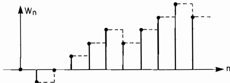
Figure 4.1 Statistical Sample of the Discrete-Time Random-Walk Process
