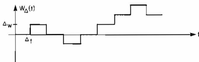
Figure 6.2 Statistical Sample of the Continuous-Time Random-Walk Process
