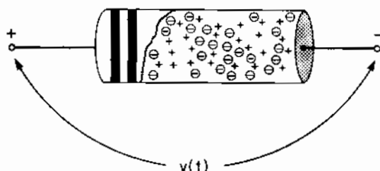
Figure 1.1 Thermal Motion of Free Electrons in a Resistor
