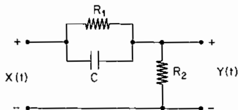
Figure 10.6 Circuit Diagram for Exercise 21
