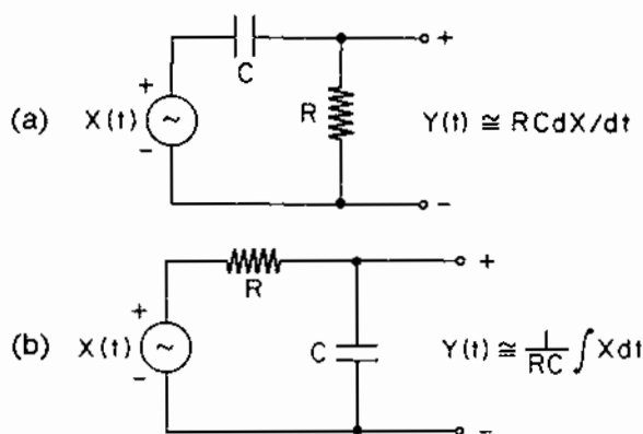
Figure 10.8 Circuit Diagrams for Exercise 10.26(a) and (b)
