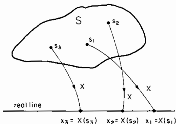
Figure 1.6 Pictorial Abstraction of a Random Variable
