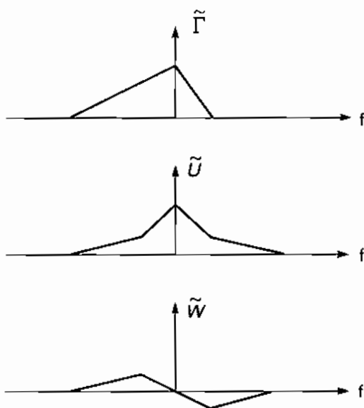
Figure 11.5 Even and Odd Symmetric Components of the Asymmetric Representation for the Case in which \tilde{\Gamma} , \tilde{U} , and \tilde{W} Are Real
