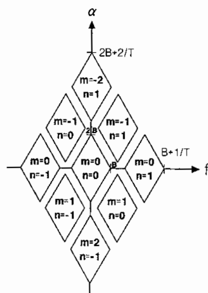
Figure 12.2 Support for the First Nine Terms in Equation (12.97) for the Cyclic Spectra of Mean-Square Bandlimited Time-Sampled Waveform for Which S_X(f) = 0 When |f| \geq B (Vertical Scale Compressed)
