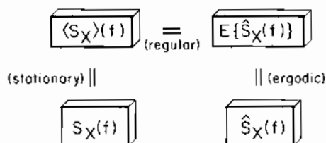
Figure 10.2 Relationships among Probabilistic and Empirical Spectral Densities
