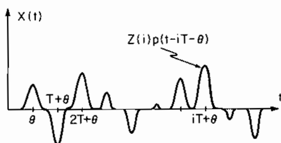
Figure 11.1 Physical Manifestation of a Discrete-Time Process
