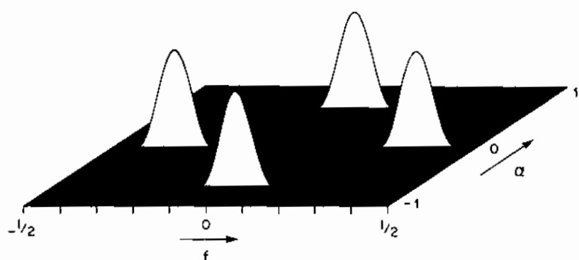
Figure 12.3 Spectral Correlation Surface for AM Signal with Stationary Amplitude
