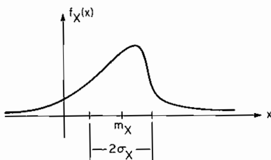
Figure 2.1 Pictorial Example of the Mean and Standard Deviation
