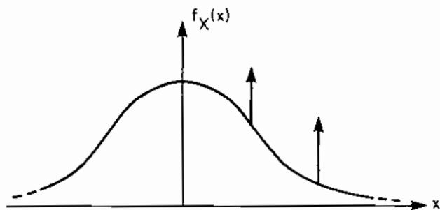
Figure 1.13 Density Function for the Mixed Random Variable in the Example Depicted in Figure 1.12
