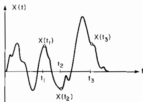
Figure 5.1 Pictorialization of Three Ordered Time Samples for the Chapman-Kolmogorov Equation
