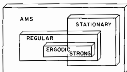
Figure 8.2 Venn Diagram of Classes of Asymptotically Mean Stationary Processes
