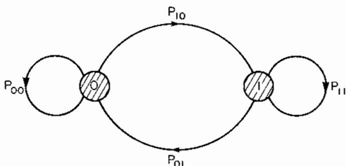
Figure 5.2 Schematic of a Two-State Markov Chain
