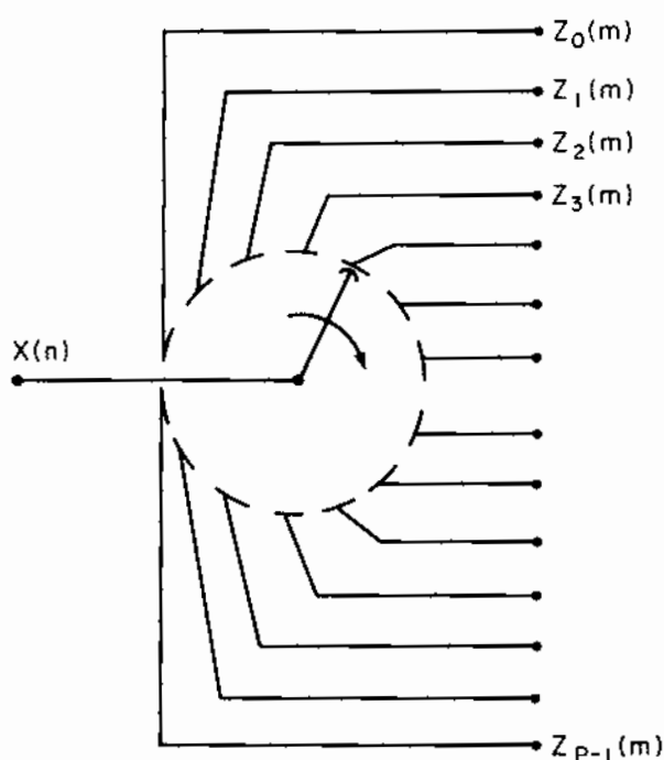
Figure 12.6 Decomposition of Cyclostationary Process into Stationary Components by Time-Division Demultiplexing Operation
