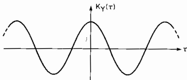
Figure 4.2 Autocovariance of the Random-Amplitude-and-Phase Sine-Wave Process mean and autocorrelation for X(t) (Section 4.2.4):
