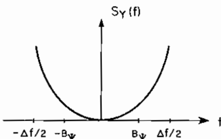
Figure 11.6 Power Spectral Density for Noise at the Output of an FM Demodulator
