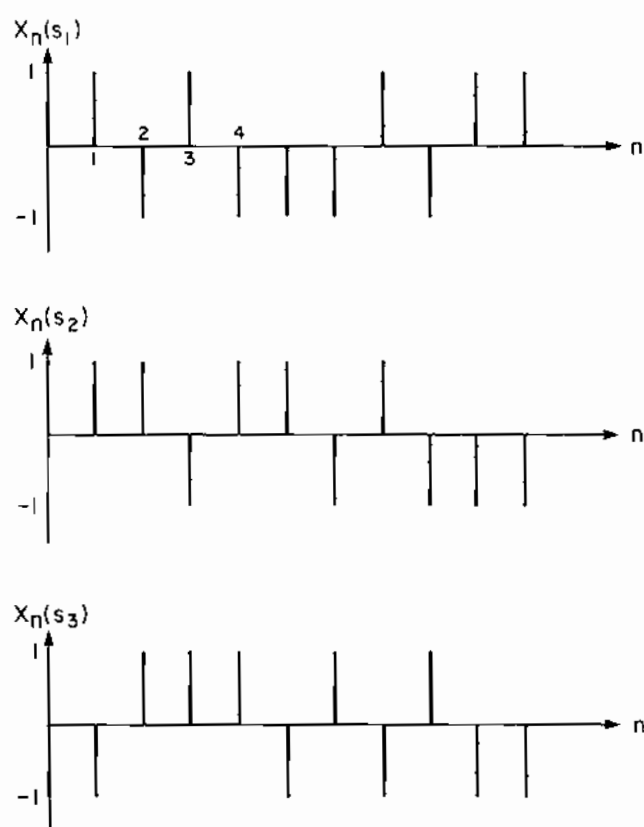
Figure 3.6 Statistical Samples of a Discrete-Valued, Discrete-Time Random Process
