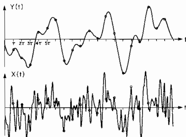
Figure 3.1 Thermal-Noise Voltage Waveforms at Low and High Temperatures: Narrowband and Broadband Frequency Compositions
