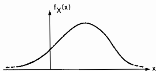
Figure 1.8 Example of a Probability Density Function
