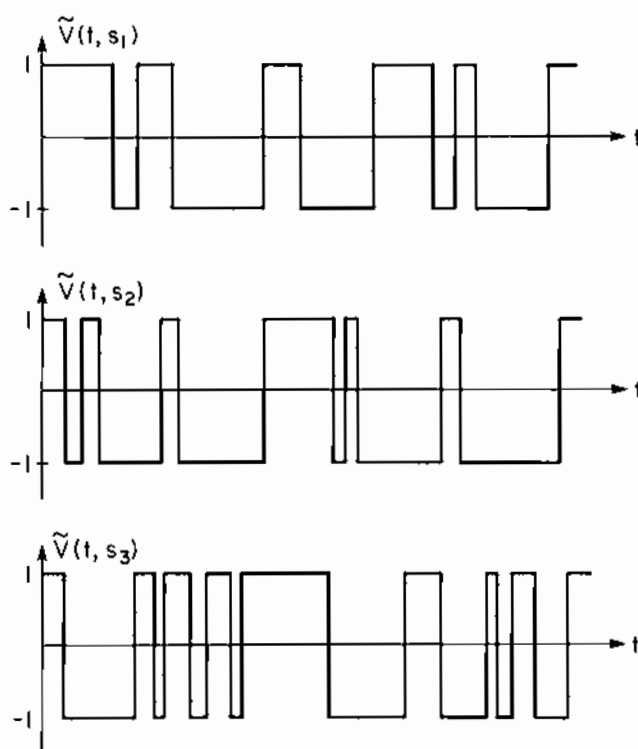
Figure 3.5 Statistical Samples of a Discrete-Valued, Continuous-Time Random Process
