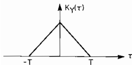
Figure 4.4 Autocovariance of the Phase-Randomized Sample-and-Held Noise Process
