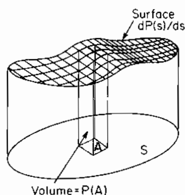
Figure 1.5 Geometrical Illustration of Probability as a Volume
