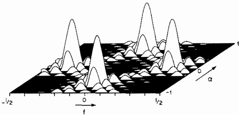
Figure 12.5 Typical Spectral Correlation Surface for BPSK Signal with Relatively Broadband Stationary Phase Sequence
