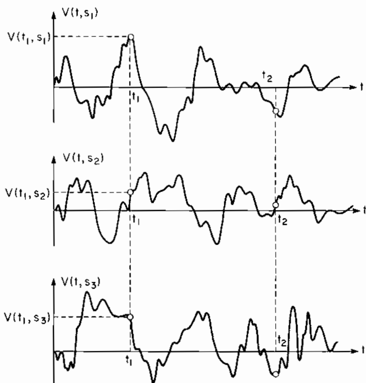
Figure 3.3 Statistical Samples of a Continuous-Time Random Process
