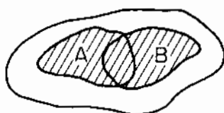
(b) Set union
