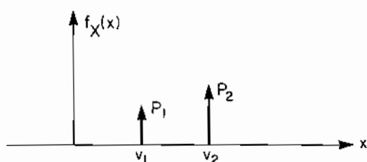
Figure 1.11 Density Function for the Discrete Random Variable in the Battery Example Depicted in Figure 1.9
