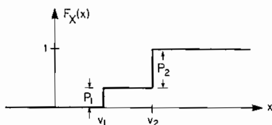
Figure 1.10 Distribution Function for the Discrete Random Variable in the Battery Example Depicted in Figure 1.9
