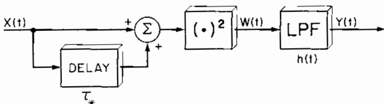
Figure 8.4 A Method for Measuring Autocorrelation
