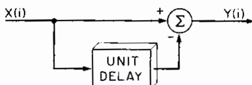
Figure 9.2 Block Diagram for Example 1
