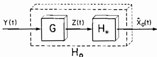
Figure 13.6 Causal Wiener Filter H_o , Decomposed into Whitening Filter G and Optimum Filter H_* for White Observations
