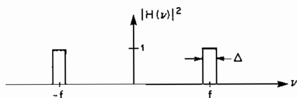
Figure 3.7 Bandpass Filter for Determination of Spectral Density
