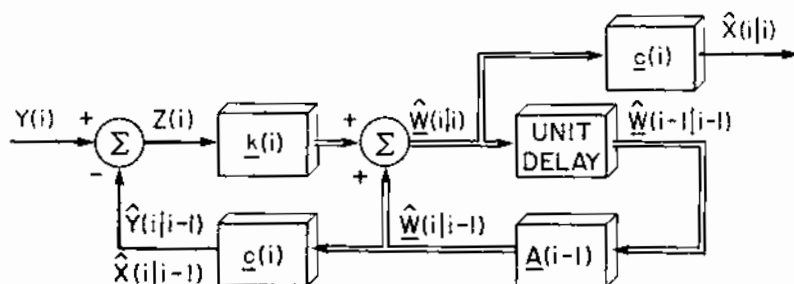
Figure 13.8 Signal-Flow Diagram for Kalman Filter
