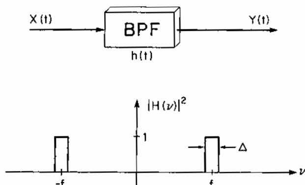
Figure 10.1 Bandpass Filter for Determination of Spectral Density
