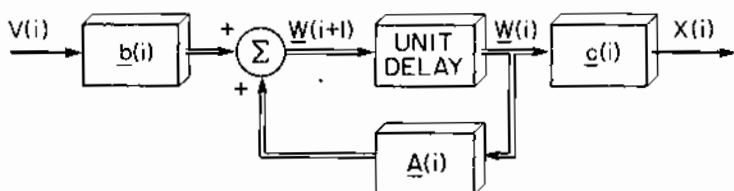
Figure 13.7 Signal-Flow Diagram for Signal-Generating Mechanism for Kalman Filtering
