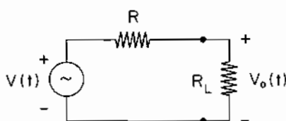
Figure 11.9 Circuit for Determining Available Power
