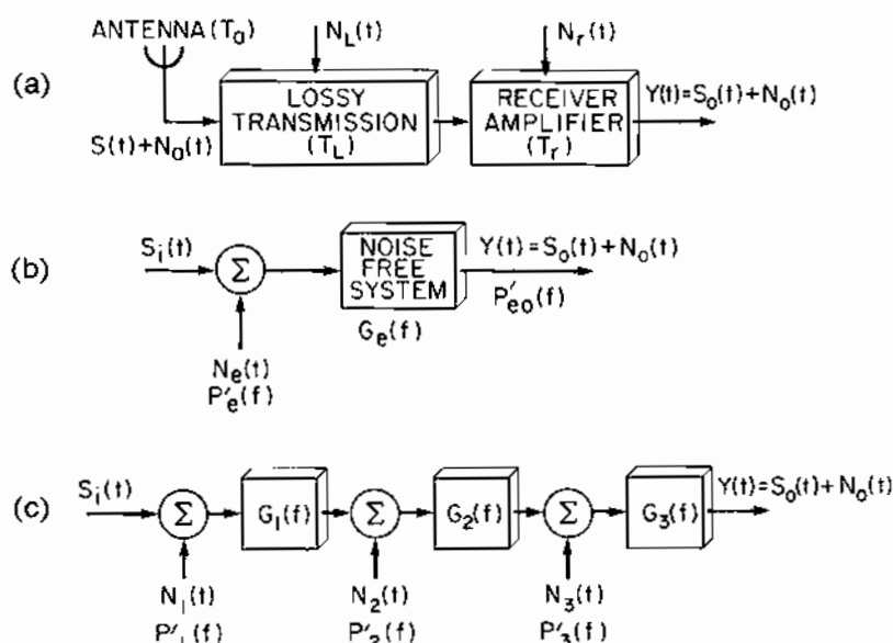
Figure 11.8 (a) Receiving System; (b) Equivalent Model of Receiving System; (c) Intermediate Equivalent Model
