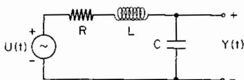
Figure 9.8 Circuit Diagram for Exercise 22
