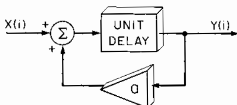
Figure 9.3 Block Diagram for Example 2
