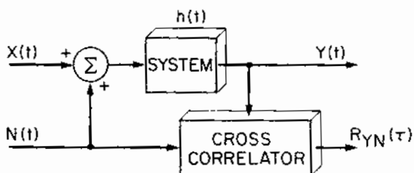
Figure 9.7 Method for Measuring the Impulse-Response Function of a Linear Time-Invariant System While It Is in Operation
