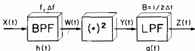
Figure 11.7 PSD Measurement System
