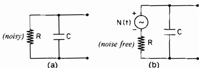
Figure 10.4 (a) Circuit for Example 4; (b) Equivalent Circuit for Example 4
