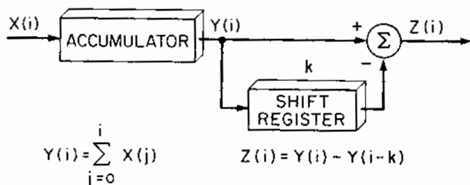
Figure 10.5 System Diagram for Exercise 11
