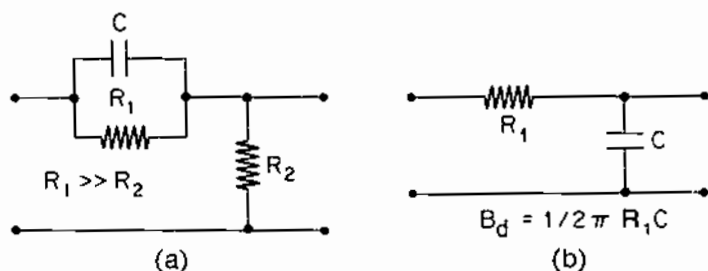
Figure 11.12 (a) Pre-emphasis Circuit for FM; (b) De-emphasis Circuit for FM
