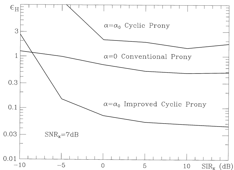
Figure 13: Sample-mean-normalized integrated squared error of the reconstruction of the multipath-channel transfer function versus signal-to-interference ratio at the channel input (the cyclic methods work at \alpha = \alpha_0 ).
