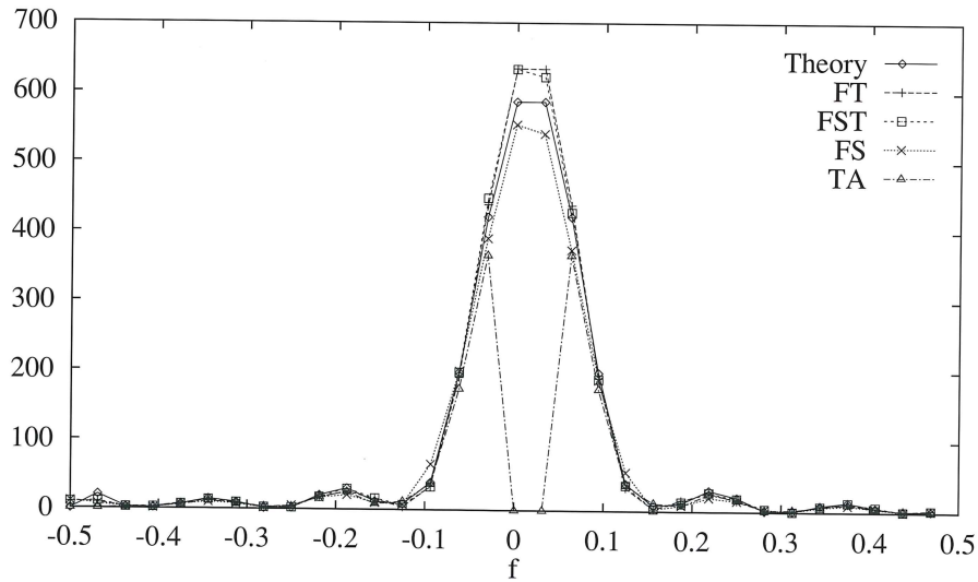
Figure 5: Estimates of the fourth-order CP for binary PAM with rectangular pulses for \beta = 0 , a collect time of 292T_0 , and f \in S_1 .
