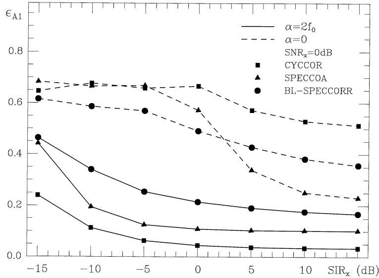
Figure 9: RMSE of the estimate of SA A_1 versus signal-to-interference ratio at the channel input for the CYCCOR, SPECCOA, BL-SPECCORR, and their corresponding GCC methods in the presence of both independent AWGNs and correlated interferences.
