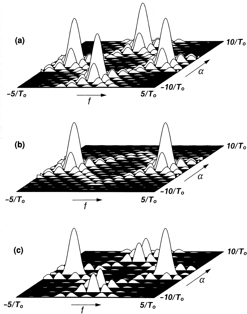
Figure 20: Magnitude of spectral correlation densities. (a) BPSK, (b) QPSK, and (c) SQPSK. (Each signal has a rectangular keying envelope.)
