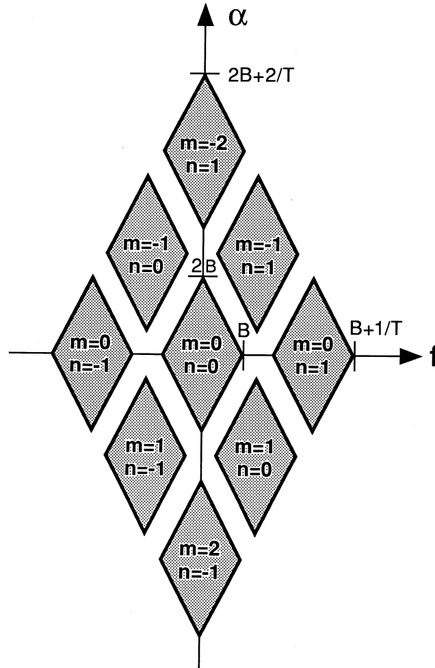
Figure 16: Illustration of support regions in the bifrequency plane for the spectral correlation densities that are aliased by periodic time sampling.
