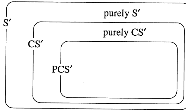
Figure 3: Venn diagram for previously defined classes of time-series.
