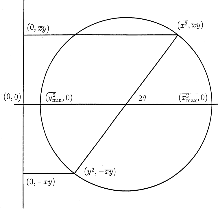
Figure 6: Relationship between the variances \overline{x^2} = \mathbf{E}\{x^2\} and \overline{y^2} = \mathbf{E}\{y^2\} and covariance \overline{xy} = \mathbf{E}\{xy\} of the amplitudes of the in-phase and quadrature components and the extrema of the variances \overline{x^2}_{\max} = \mathbf{E}\{x^2\}_{\max} and \overline{y^2}_{\min} = \mathbf{E}\{y^2\}_{\min} attainable by shifting the reference phase of the filter output.
