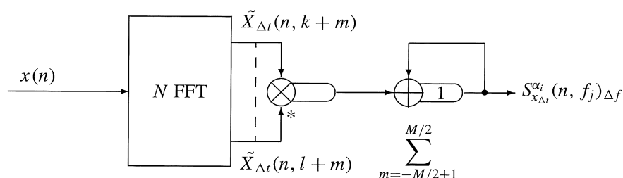
Figure 8: Digital implementation of the Direct Frequency Smoothing Method.
