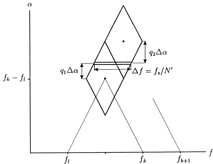
Figure 4: Adjacent cell combining for mitigation of variable frequency resolution in the FAM.
