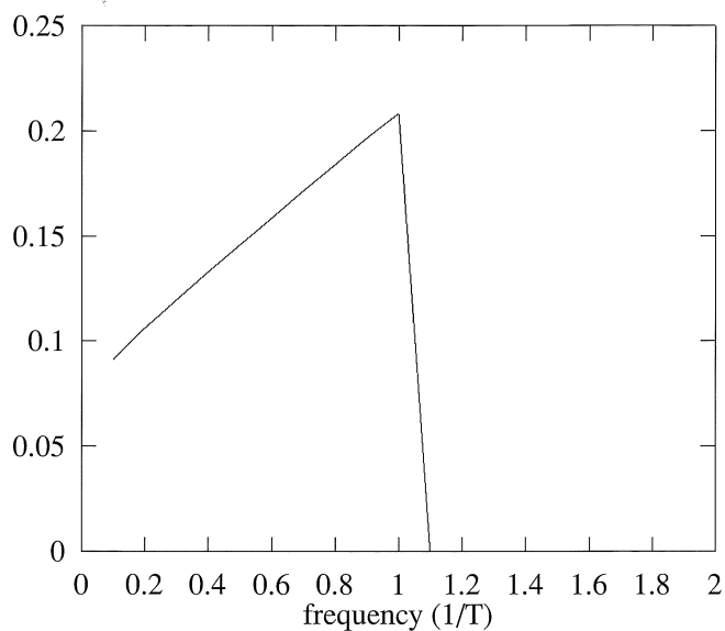
(a) Optimal Transmitter for Un-coordinated Case ( L=1 )
