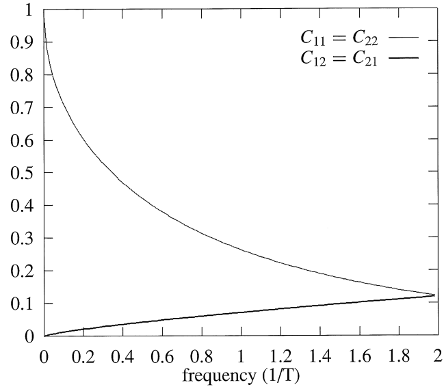
(a) Channel Response
