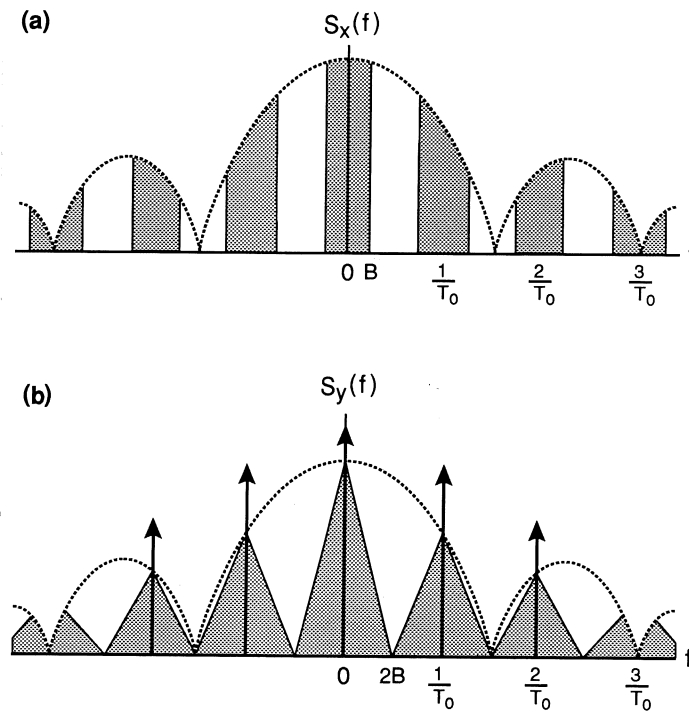
Figure 7: (a) Power spectral density (PSD) of a pulse-amplitude-modulated (PAM) signal with 67% duty-cycle pulses. (b) PSD of the squared PAM signal.
