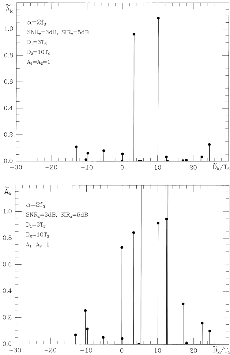
Figure 10: (a) SA and AT estimates by the improved cyclic Prony method working at \alpha = 2f_0 . (b) SA and AT estimates by the cyclic Prony method working at \alpha = 2f_0 . (c) SA and AT estimates by the conventional Prony method.
