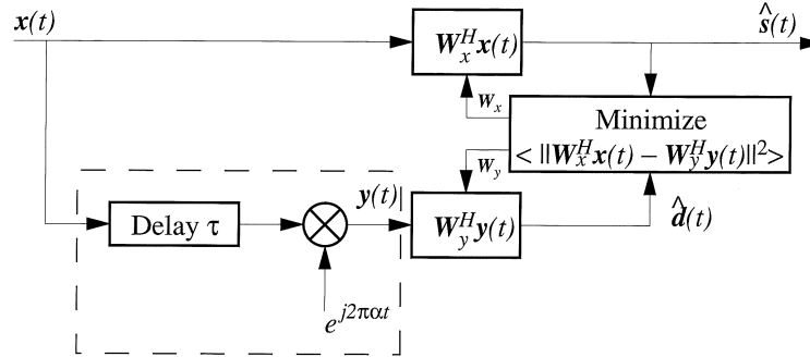
Figure 6: Block diagram of Cross-SCORE processor.
