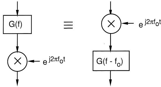
Figure 2: Input/output equivalent subsystems that employ exponential modulators.
