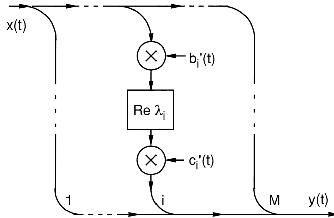
Figure 3: Canonical configuration for M -th order PTV system.
