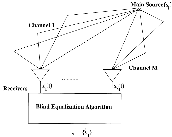
Figure 5: An antenna-array-based blind equalizer.
