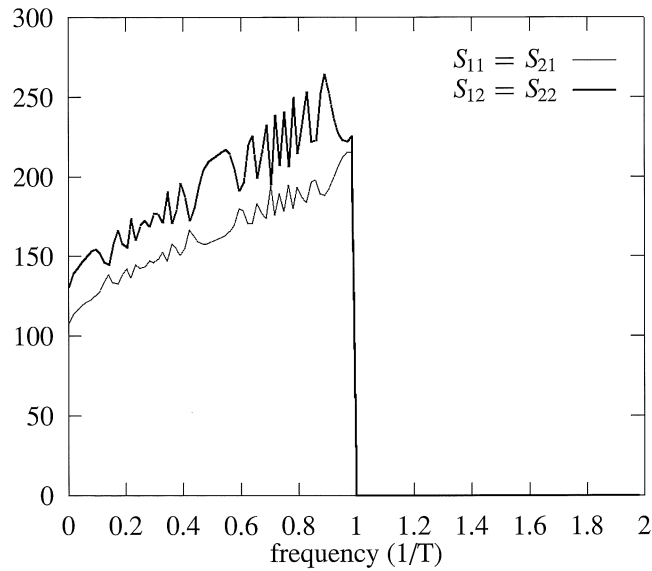
(b) Optimal Transmitter for Co-Ordinated Case
