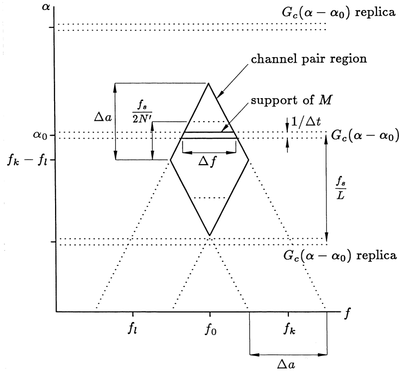
Figure 3: Region-of-support diagram for the FFT Accumulation Method.
