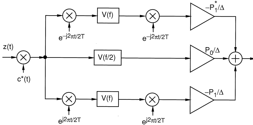
Figure 7: Optimum demodulation filter for spread-spectrum signal at high SNR. \Delta = P_0^2 - |P_1|^2 .
