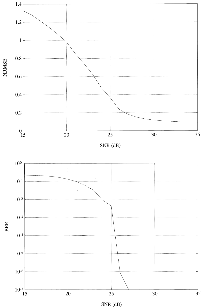
Figure 4: (a) NRMSE vs. SNR for 100 Monte Carlo runs with 100 symbols used for channel estimation in each run. (b) BER vs. SNR for 100 Monte Carlo runs with 100 symbols used for channel estimation in each run.
