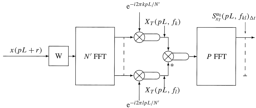
Figure 5: Digital implementation of the FFT Accumulation Method.
