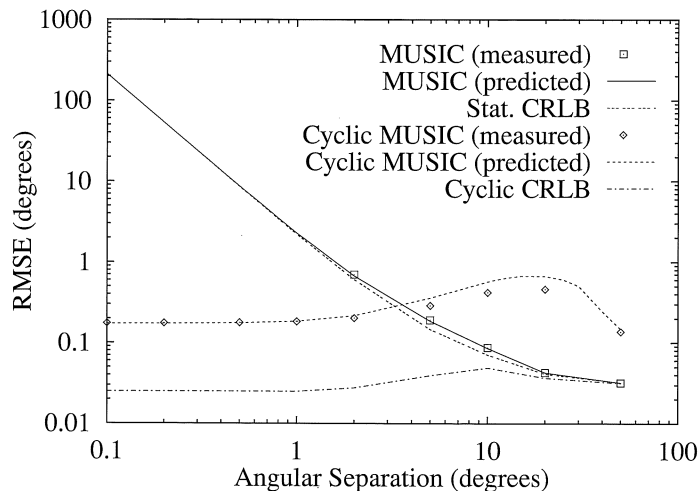
Figure 16: RMSE as a function of angular separation for one SOI with 10 dB SNR in the presence of 1 equal-powered SNOI and complex white Gaussian noise.
