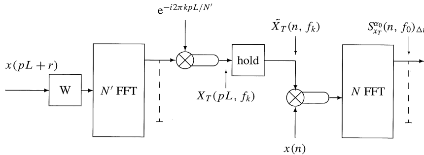
Figure 6: Digital implementation of the Strip Spectral Correlation Algorithm.
