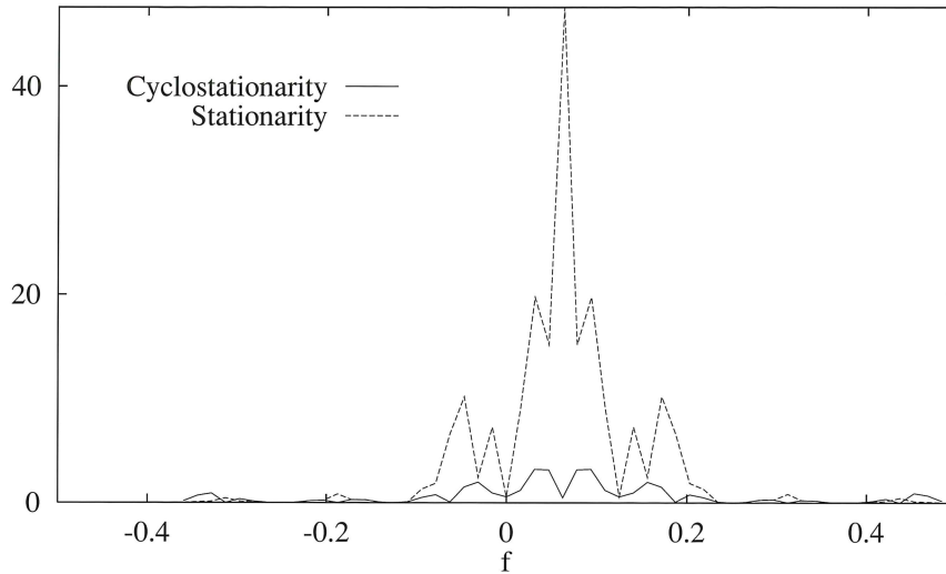
Figure 9: The fourth-order CP for a binary PAM signal under the assumptions stationarity and cyclostationarity.
