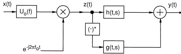
Figure 8: Complex envelope transformation followed by LCL processing.
