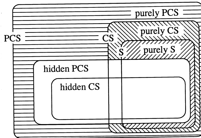
Figure 4: Venn diagram of classes of stochastic processes.
