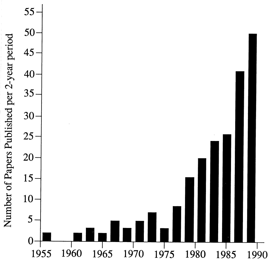
Figure 1: Histogram of papers on cyclostationarity.
