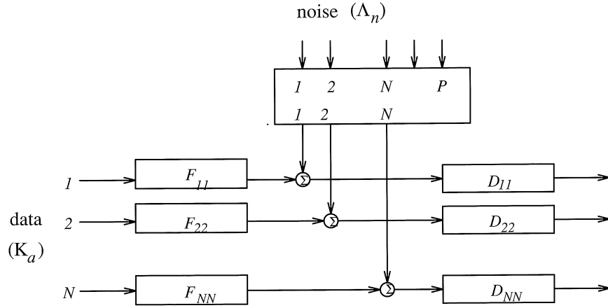
Figure 4: Optimal transmitter and receiver filter structure.
