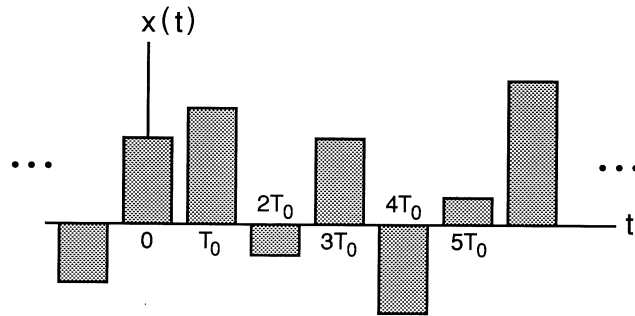
Figure 6: A pulse-amplitude-modulated (PAM) signal with pulse width less than interpulse time.
