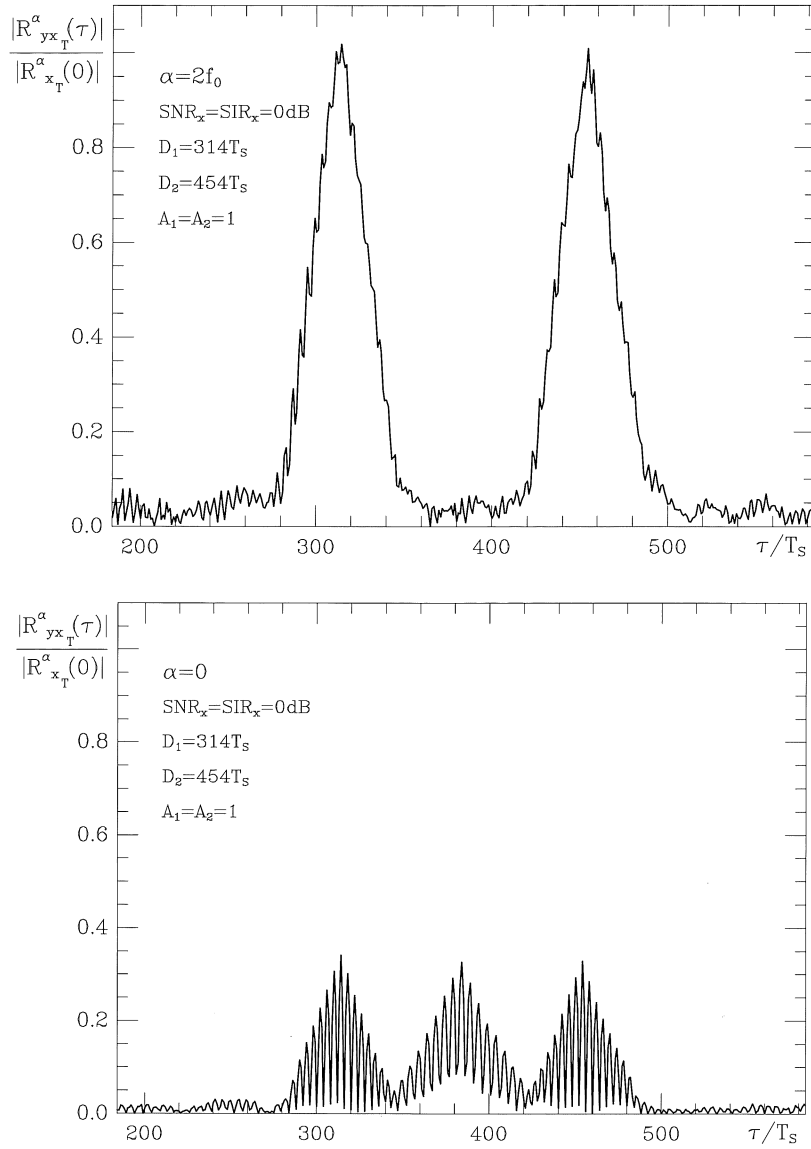
Figure 1: (a) Graph of magnitude of normalized cyclic cross-correlogram. (b) Graph of magnitude of normalized cross-correlogram.
