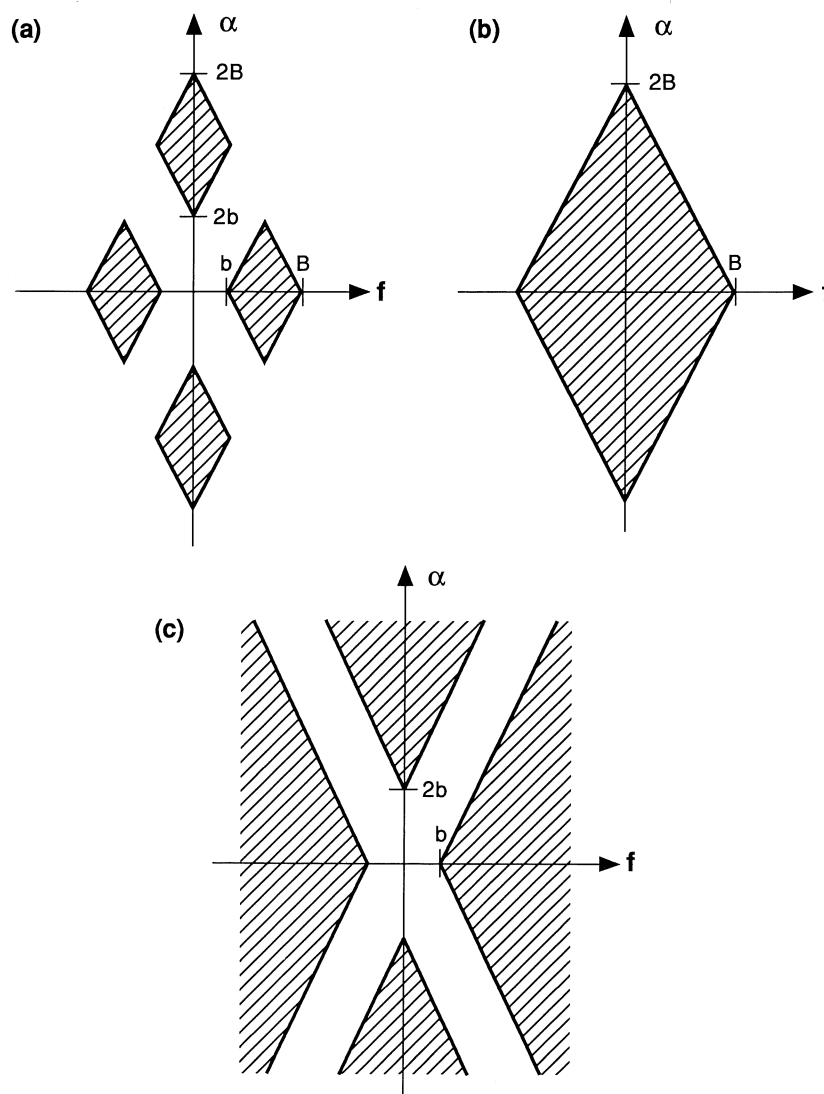
Figure 14: (a) Support region in the bifrequency plane for the spectral correlation density function of a bandpass signal. (b) Support region for a lowpass signal. (c) Support region for a highpass signal (shown over a small fraction of the diamond-shaped principal domain).
