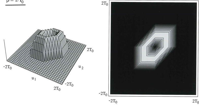
Figure 2: Surface and contour plots of the theoretical RD-CTCF for a real-valued binary PAM signal with a rectangular pulse shape.
