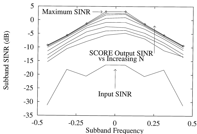
Figure 14: Average SINR (averaged over 100 trials) in each of the 8 subbands of SCORE processor output, plotted for different numbers N of data samples: 128, 256, 512, ..., 8192. The input SINR at the first sensor and the maximum-attainable output SINR are shown at the extreme bottom and top of the graph, respectively.
