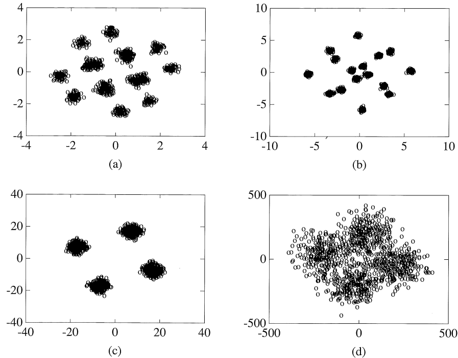
Figure 6: Constellations for SNR = 20 dB with 20 symbols used for channel estimation. (a) Unequalized output of receiver no. 1. (b) Unequalized output of receiver no. 2. (c) Equalized output using three receivers. (d) Equalized output using receiver no. 1.
