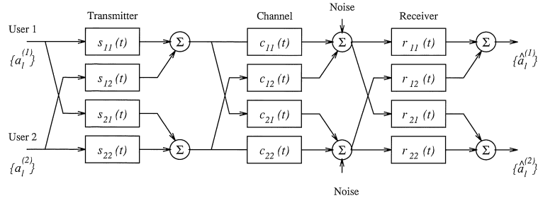
Figure 2: Coordinated MIMO system ( N = P = 2 ).
