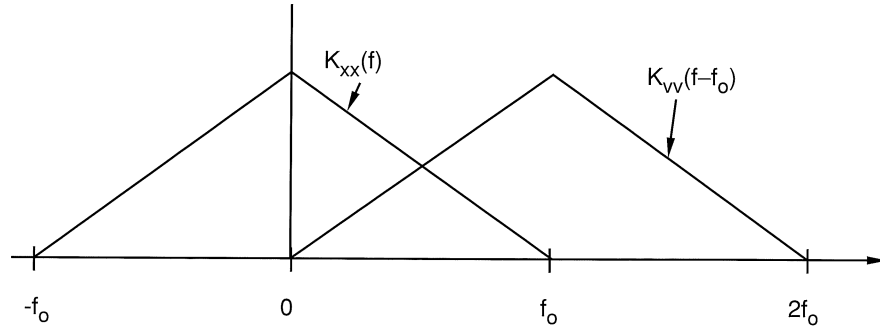
Figure 9: Example involving two interfering DSB signals.
