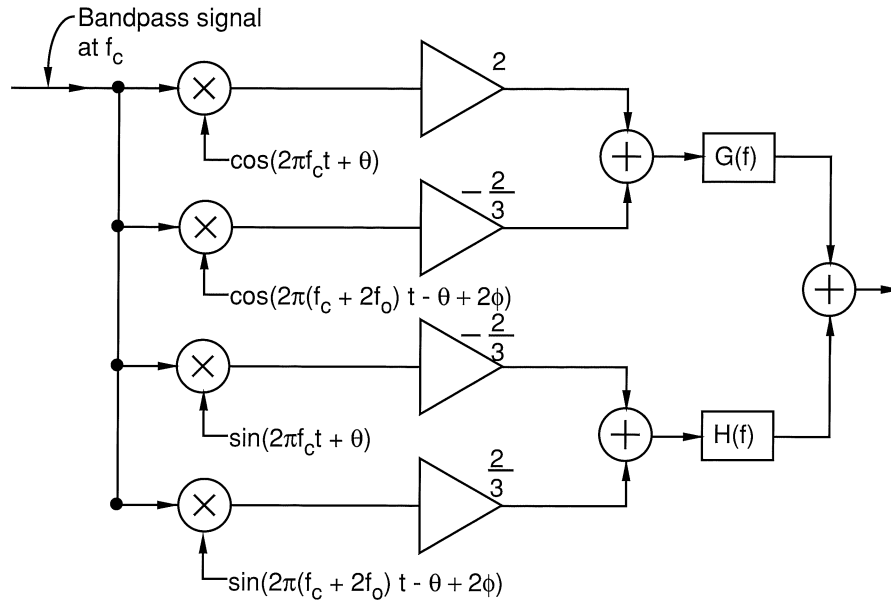
Figure 10: Optimum linear demodulator for DSB signal with upper-sideband co-channel interference and high SNR.
