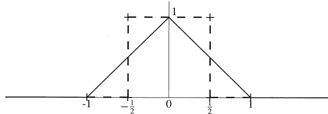
Figure 2: The rect (dashed) and \Lambda (solid) functions.
