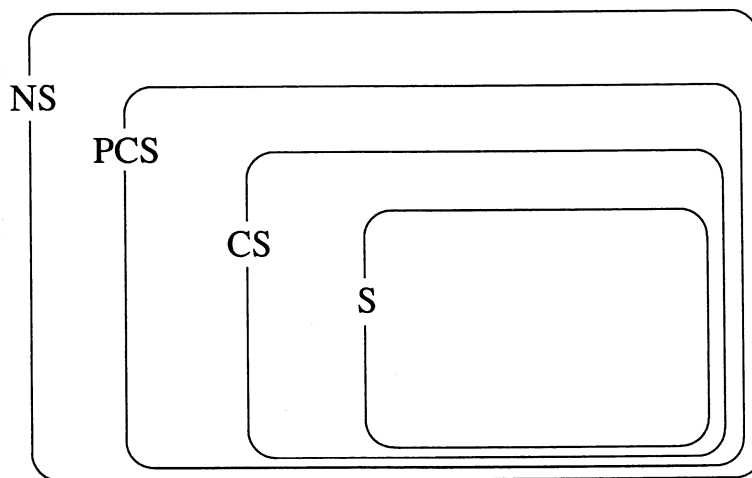
Figure 2: Venn diagram of classes of stochastic processes. With the class NS omitted, also the Venn diagram of classes of time-series.
