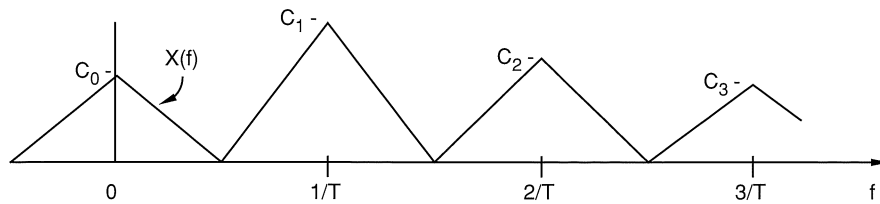
Figure 6: Spectrum of spread signal.
