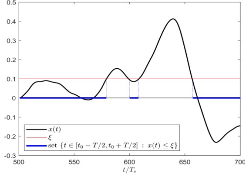
Fig. 1 The measure of the set \{t \in [t_0 - T/2, t_0 + T/2] : x(t) \leq \xi\} (blue thick line) normalized by the total time T is the fraction of time that the function x(t) is below the threshold \xi as t ranges over [t_0 - T/2, t_0 + T/2] .
