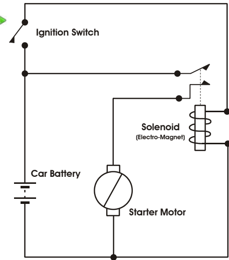
Car starter switching circuit © author
