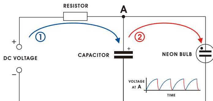
Circuit of a simple relaxation oscillator © author
