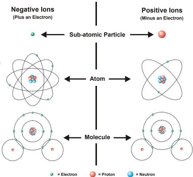
Electrons, Ionised Atoms and Molecules © author
