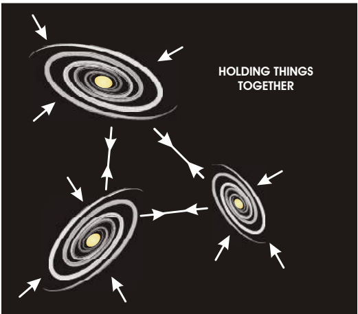
Galaxies and the Stars inside being held together © author
