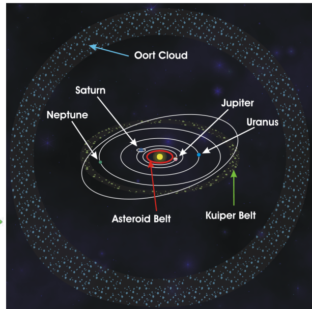
The Oort Cloud, Kuiper Belt and Asteroid Belt in relation to the Solar System © author
