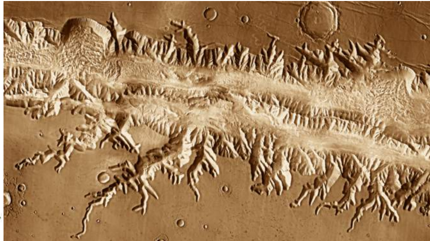
Valles Marineris on Mars Credit NASA/JPL MRO
