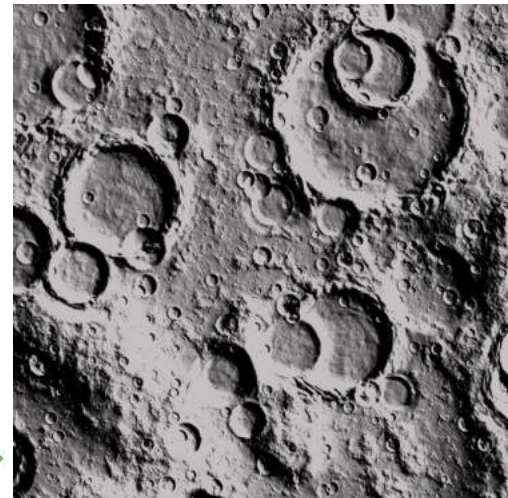
Moon craters - some in twos and threes - Credit NASA
