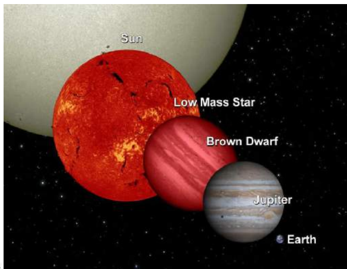
A comparison of star and planet sizes to Earth Credit: NASAJPL-CaltechUCB ▶
