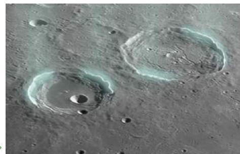
The action of electrical erosion on craters (Conceptual) - Original Image Credit NASA
