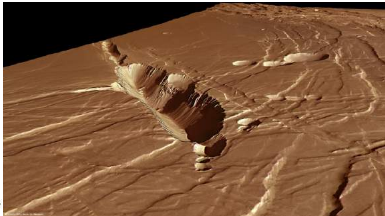
Phoenixis Lacus Rille on Mars Credit ESA/DLR/FU Berlin (G. Neukum) ▲
