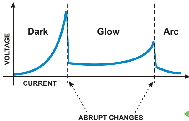
The three plasma states © author
