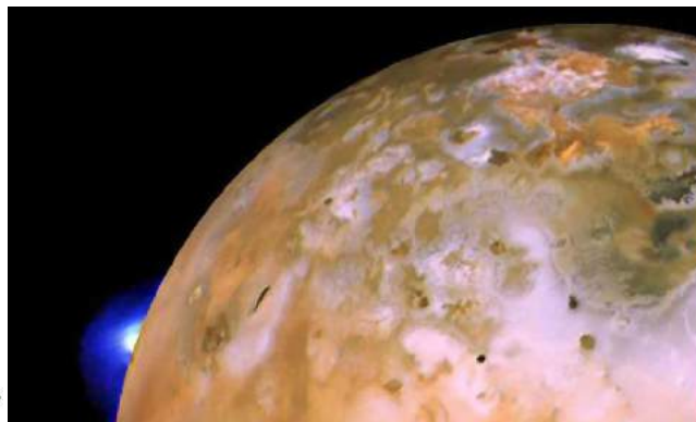
Jupiter's moon Io and the 'erupting' volcano Loki Credit: NASA JPL USGS
