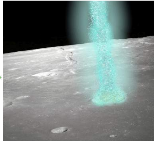
Birkeland Current scouring out a Crater on the Moon Original Image Credit: NASA
