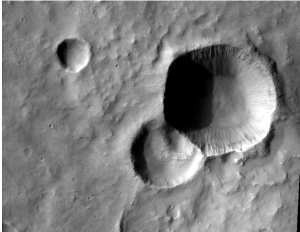
◀ Themis Crater on Mars - Image courtesy NASA/JPL-Caltech/ASU
