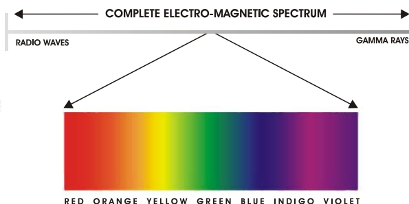
The visible portion of the Electro-Magnetic Spectrum © author ▶
