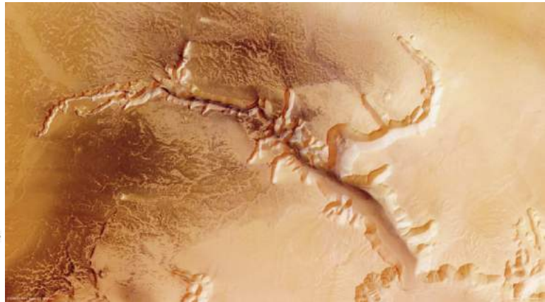
Echus Chasma (1) Rille on Mars Credit ESA/DLR/FU Berlin (G. Neukum) ▶
