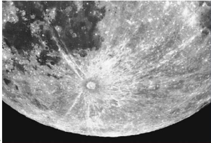
The Moon's crater Tycho and its 'Rays' - Credit NASA HST
